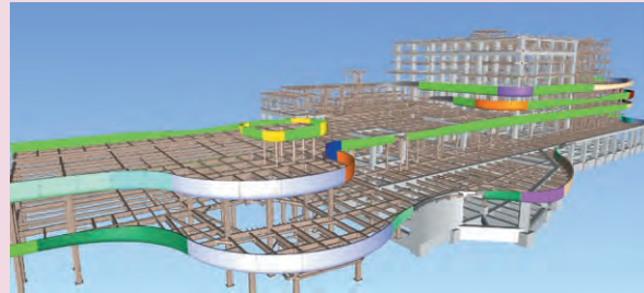
鉄骨取合い検討(Navisworks)
